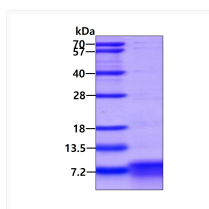
SDS-PAGE gel of recombinant human alpha-Synuclein 1-95aa protein under reducing conditions Coomassie stain
