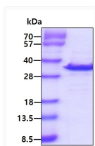
SDS-PAGE gel showing recombinant human SHP-1 protein 3 µg under reducing conditions with Coomassie blue staining
