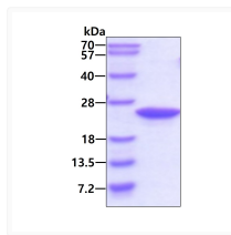
SDS-PAGE gel showing recombinant human RBP4 protein 3µg under reducing conditions Coomassie blue stain
