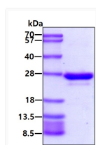
SDS-PAGE of recombinant human RAB5A protein under reducing conditions
