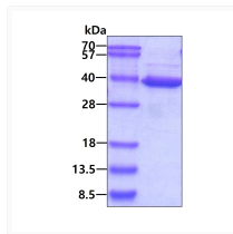
SDS-PAGE gel of recombinant human PTP1B protein 3µg under reducing conditions stained with Coomassie blue
