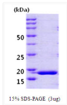
SDS-PAGE of recombinant human Cyclophilin H PPIH protein under reducing conditions
