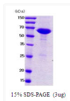
SDS-PAGE gel of recombinant E.coli NusA protein 3µg under reducing conditions Coomassie blue stain
