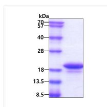
SDS-PAGE of recombinant human IL-16 protein under reducing conditions Coomassie blue stain
