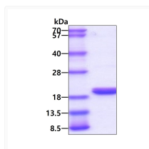
SDS-PAGE of recombinant human IL-1Ra IL1RN protein under reducing conditions Coomassie blue stain
