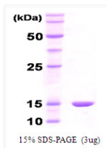
SDS-PAGE gel of recombinant E. coli GroES protein under reducing conditions
