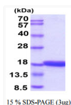
SDS-PAGE of recombinant human GADD45 beta protein under reducing conditions with Coomassie blue staining
