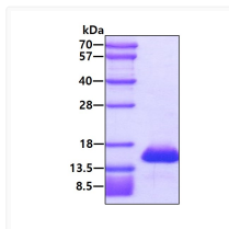
SDS-PAGE gel showing 3µg recombinant human FABP5 E-FABP protein under reducing conditions Coomassie blue stain
