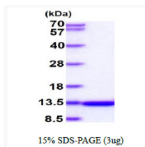
SDS-PAGE gel of recombinant human FABP6 protein under reducing conditions with Coomassie blue stain
