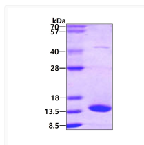
SDS-PAGE gel of recombinant human FABP7 B-FABP protein STJP019619 under reducing conditions
