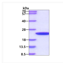
SDS-PAGE gel of recombinant human Cyclophilin B PPIB protein under reducing conditions
