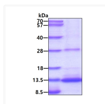
SDS-PAGE gel of recombinant human BMP-2 monomer protein under reducing conditions Coomassie stain
