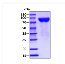
SDS-PAGE gel of recombinant human GFR alpha-1 protein under reducing conditions stained with Coomassie blue
