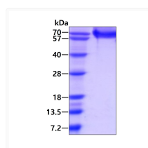
SDS-PAGE of recombinant human IBSP Sialoprotein II protein under reducing conditions
