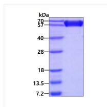
Recombinant mouse CD99-L2 protein SDS-PAGE gel under reducing conditions stained with Coomassie blue
