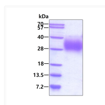
Recombinant human TREM2 protein SDS-PAGE gel under reducing conditions with Coomassie blue stain
