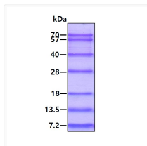
NKMAX Protein Marker 7 bands SDS-PAGE gel under reducing conditions stained with Coomassie blue
