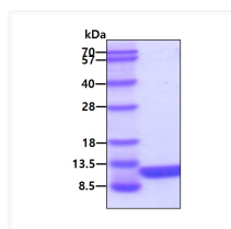
SDS-PAGE of recombinant human Resistin RETN protein under reducing conditions with Coomassie blue stain
