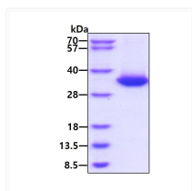
SDS-PAGE gel of recombinant human Kallikrein 3 PSA protein under reducing conditions
