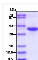
SDS-PAGE gel of recombinant human NQO1 protein under reducing conditions stained with Coomassie blue
