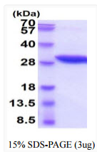
SDS-PAGE gel of recombinant mouse NNMT protein under reducing conditions Coomassie stain
