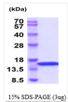
SDS-PAGE of recombinant canine IFN-gamma IFNG protein under reducing conditions
