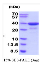
SDS-PAGE gel of recombinant human AKR1C4 protein 3µg under reducing conditions Coomassie stain
