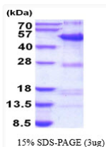
SDS-PAGE gel of recombinant human SYT11 protein under reducing conditions Coomassie blue stain
