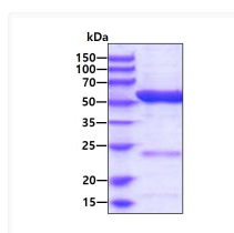
SDS-PAGE gel of recombinant human ALDH6A1 protein stained with Coomassie blue
