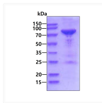
Recombinant human PNPT1 protein SDS-PAGE gel 3µg reducing conditions Coomassie stain
