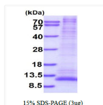
SDS-PAGE gel of recombinant human GNG12 protein under reducing conditions stained with Coomassie blue
