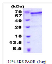
SDS-PAGE gel of recombinant human PTDSR JMJD6 protein 3µg reducing conditions Coomassie blue
