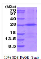
SDS-PAGE gel of recombinant human THOC7 protein under reducing conditions stained with Coomassie blue
