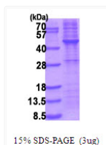
SDS-PAGE gel of recombinant human TRIB3 protein under reducing conditions with Coomassie blue stain
