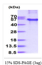
SDS-PAGE gel of recombinant human CREB3L2 protein under reducing conditions
