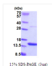
SDS-PAGE gel of recombinant human AAMDC protein 3µg under reducing conditions Coomassie blue stain
