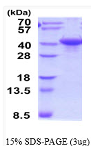
SDS-PAGE gel showing 3µg recombinant human IGSF4A CADM1 protein under reducing conditions Coomassie blue stain
