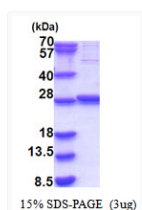
SDS-PAGE gel of recombinant human GLTPD1 protein under reducing conditions
