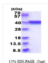
SDS-PAGE gel showing recombinant E. coli gldA protein 3 µg Coomassie blue stain
