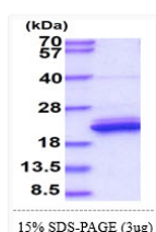
SDS-PAGE gel of recombinant human Lipocalin-1 protein under reducing conditions stained with Coomassie blue
