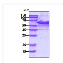
SDS-PAGE gel showing 3µg recombinant human ETS2 protein under reducing conditions stained with Coomassie blue
