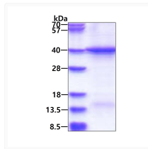
SDS-PAGE of recombinant human HERC5 protein under reducing conditions stained with Coomassie blue
