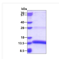
SDS-PAGE gel of recombinant human MZB1 protein under reducing conditions Coomassie blue stain
