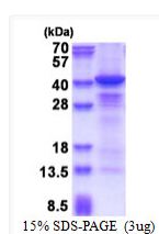
SDS-PAGE gel of recombinant human CSNK1A1 protein under reducing conditions stained with Coomassie blue
