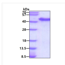
SDS-PAGE gel showing recombinant human USP46 UAF1 protein under reducing conditions stained with Coomassie blue
