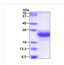
SDS-PAGE of recombinant human CHAC2 protein 3µg under reducing conditions with Coomassie blue staining
