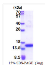
SDS-PAGE gel of recombinant human JAK2 protein under reducing conditions Coomassie blue stain
