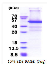
SDS-PAGE gel of recombinant human PSMD11 protein under reducing conditions stained with Coomassie blue
