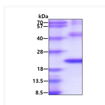
SDS-PAGE gel of recombinant human TREM2 protein under reducing conditions with Coomassie blue stain
