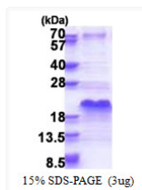
SDS-PAGE gel of recombinant human SHFM1 protein stained with Coomassie blue
